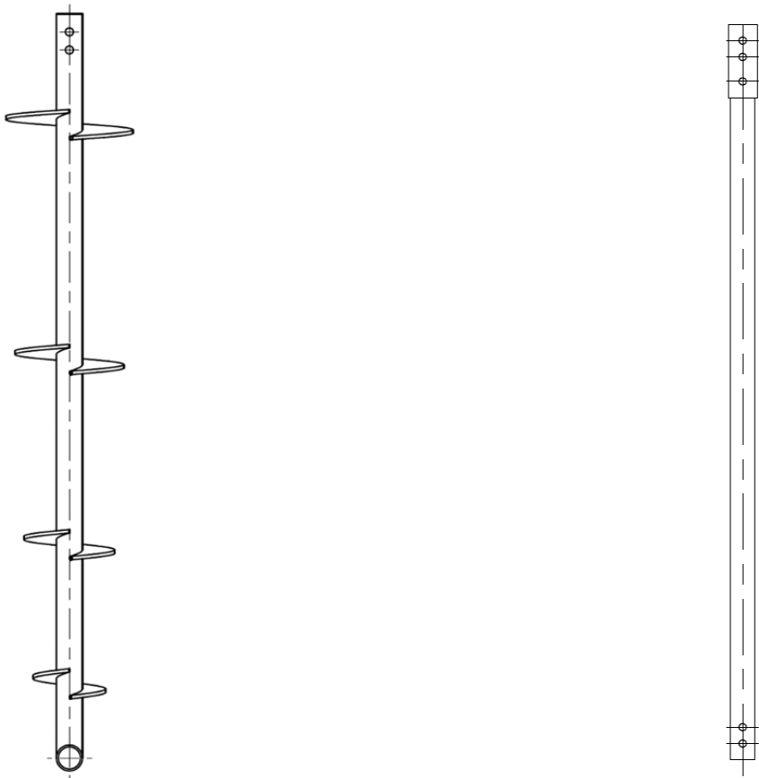
FIGURE 1—TYPICAL HELICAL PILE LEAD AND EXTENSION WITH COUPLER
