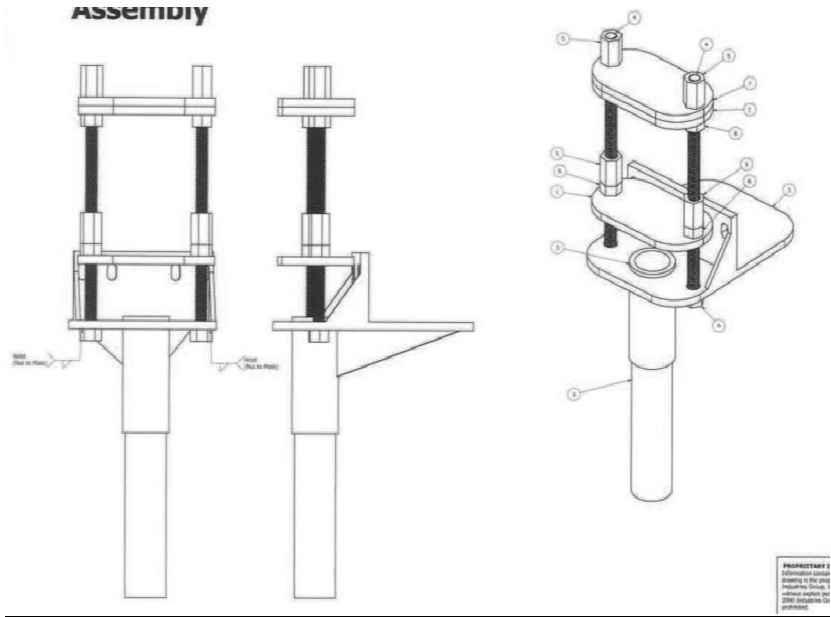
FIGURE 2—REPAIR BRACKET
